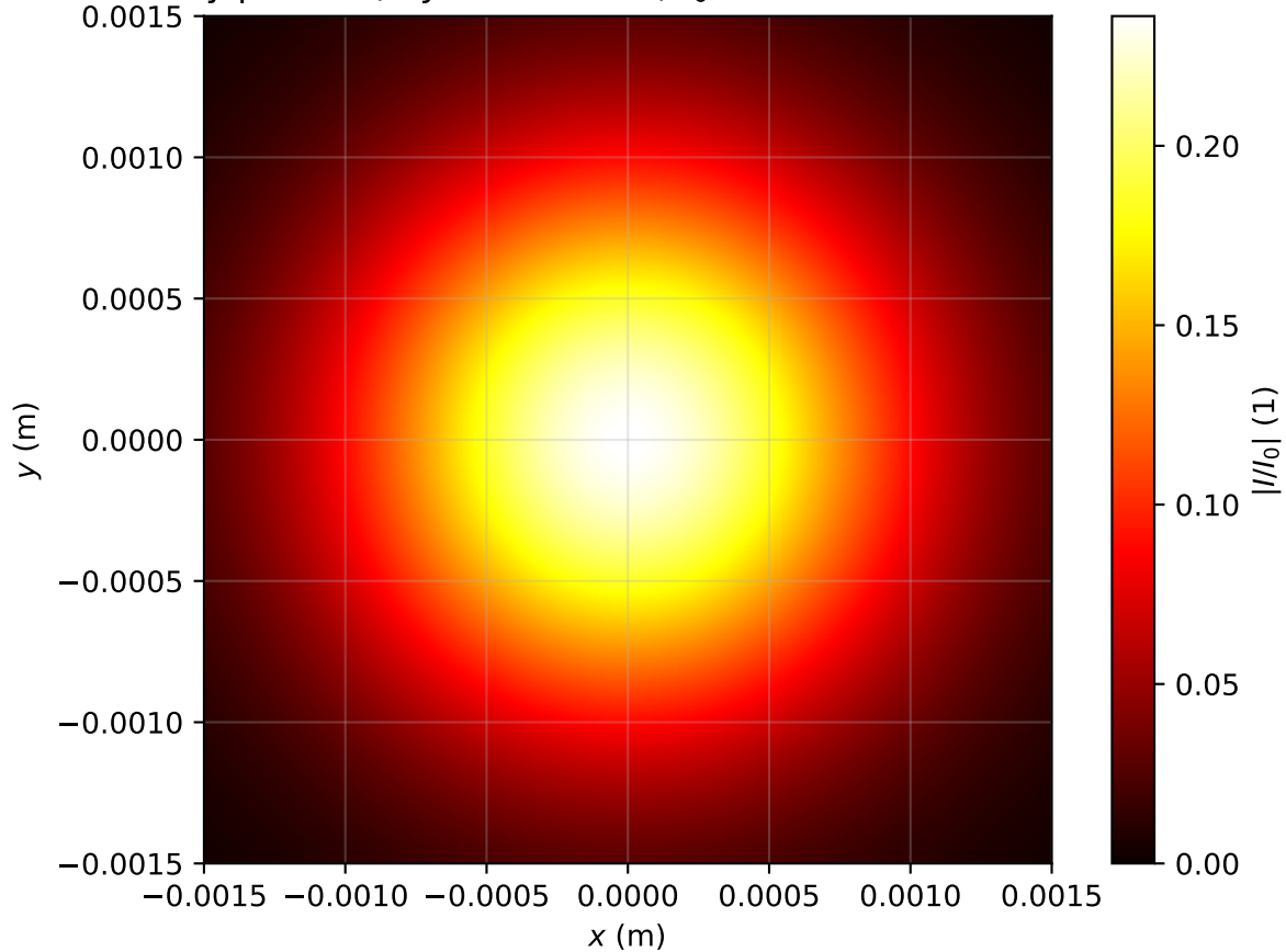
Intensity profile I(x, y, z = 3.821m)/I_0 , P_{in}=0.1P_{cr} , artificial time
